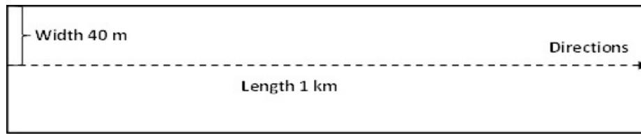
Figure 2. Transect method
