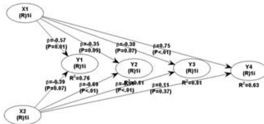
Gambar (Figure) 5. Model PLS pengaruh Y1 (jumlah klorofil a), Y2 (jumlah klorofil b), Y3 (klorofil tot) dan Y4 (indeks stomata) terhadap X1 (suhu) dan X2 (kelembapan) (PLS model) (The PLS model with Y1 (amount of chlorophyll a), Y2 (amount of chlorophyll b), Y3 (chlorophyll tot) and Y4 (stomata index) effects on X1 (temperature) and X2 (humidity) (PLS model)
