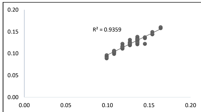
Gambar (Figure) 8. Scatter plot simulasi model debit aliran dan pengamatan pada proses validasi ( Scatter plot simulation of the flow discharge model and observations on the validation process )
