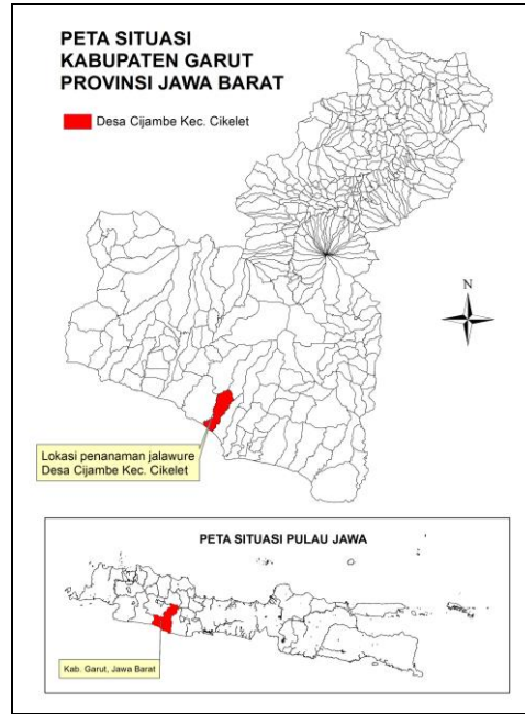
Gambar (Figure) 1. Lokasi penanaman agroforestri jati-jaluwure di Desa Cijambe Kecamatan Cikelet. (Location of teak-jaluwure agroforestry plantation in Cijambe Village, Cikelet Sub-Districts)
