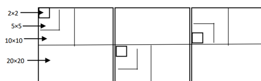
Figure 2. Vegetation analysis checkered line plot illustration
